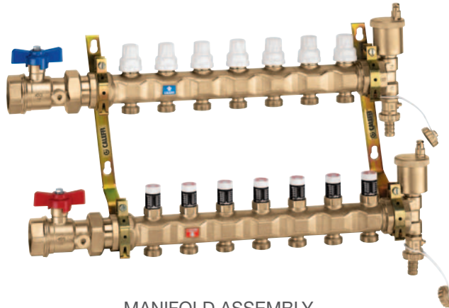
MANIFOLD ASSEMBLY
